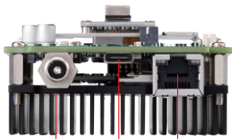
DC 12~24V For kit LAN USB Type-C (power for kit, HDMI and USB)
